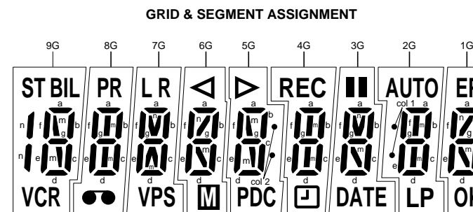
A7001 DISPLAY (FLD) GRID / ANODE ASSIGNMENT DRAWING & TABLE
